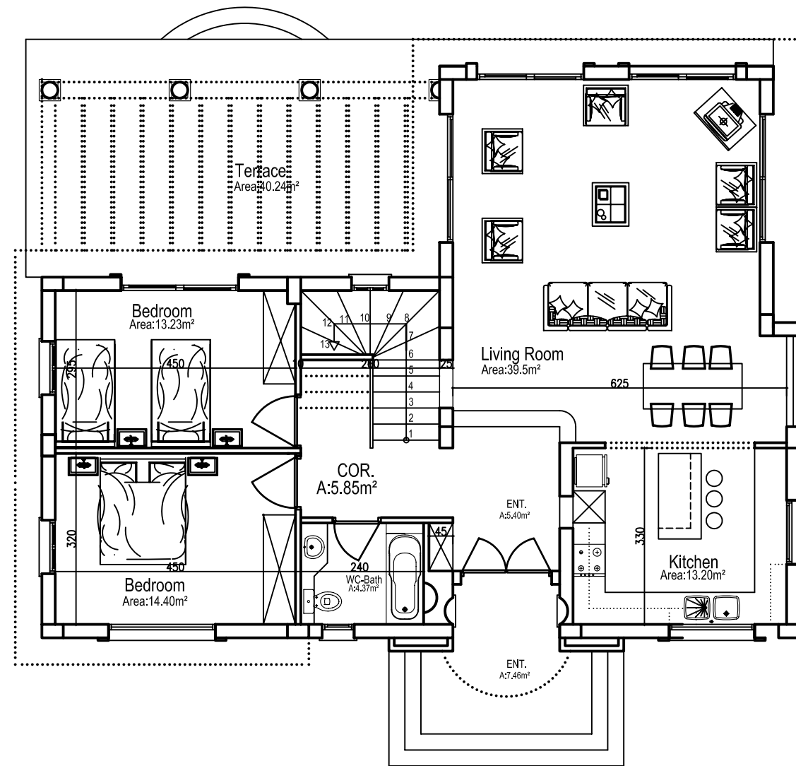
GROUND FLOOR PLAN Total Area: 121.5m 2
